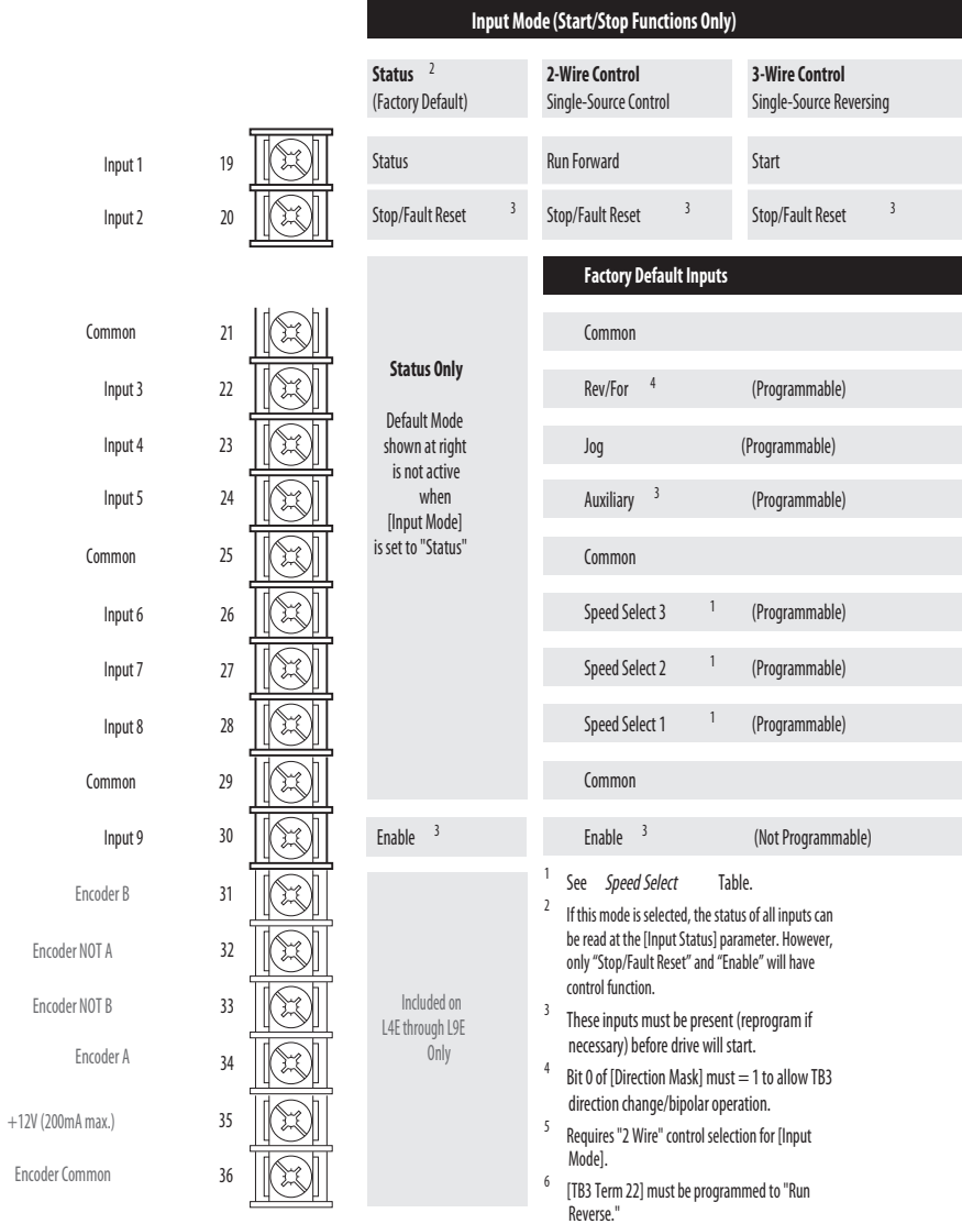
Figure 46 - 1336 PLUS II Drive TB3 Digital I/O Default Settings
