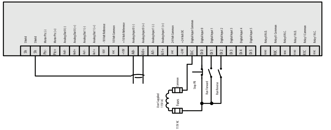
Figure 71 - 2-wire Control, Analog Input Reference Wiring Example
