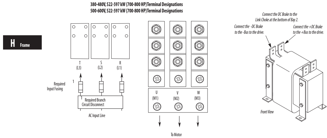
Figure 33 - 1336 IMPACT Drive Power Terminal Blocks (H)
