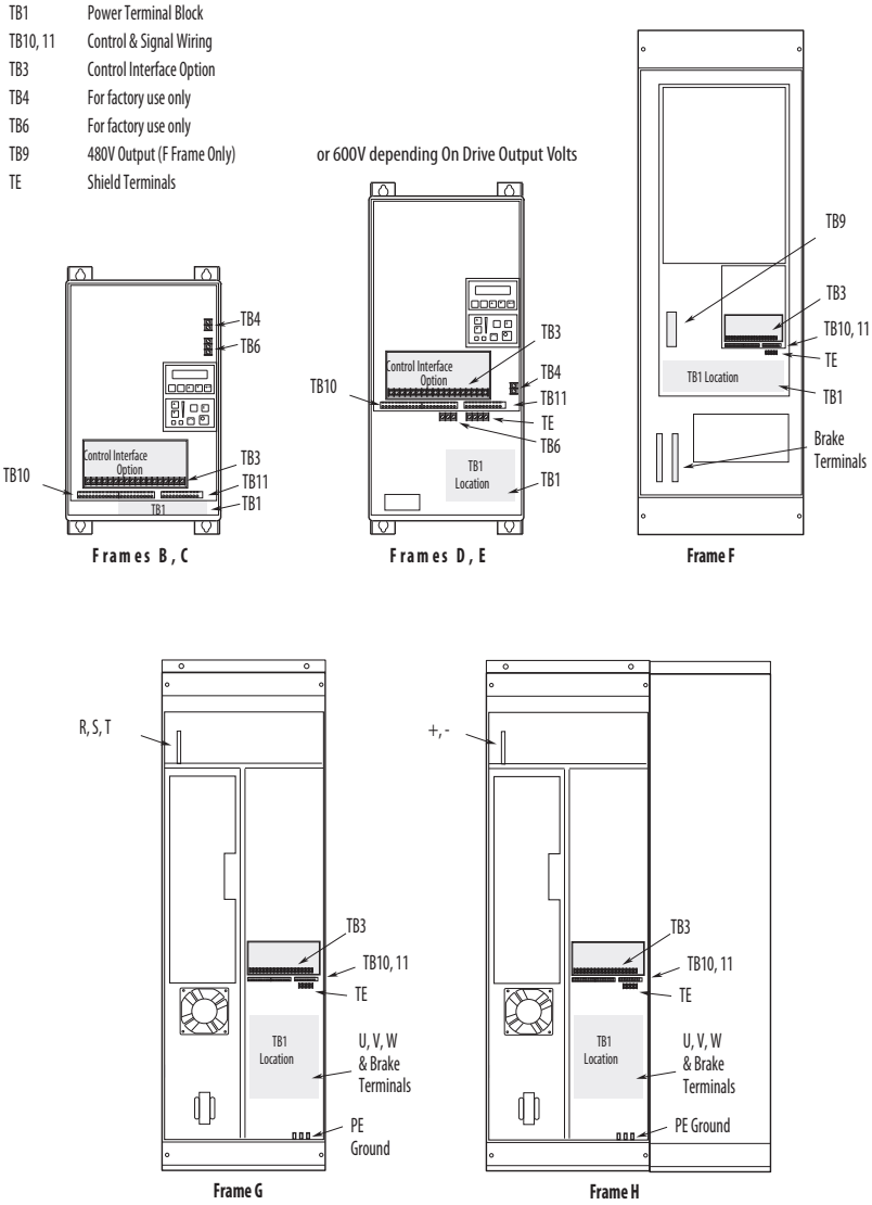
Figure 29 - 1336 IMPACT Drive Power Terminal Block Locations (B...H)
