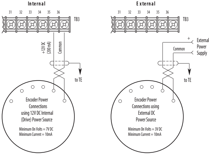
Figure 55 - Encoder Power Wiring
