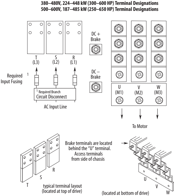
Figure 26 - 1336 FORCE Drive Power Terminal Blocks (G, H)
