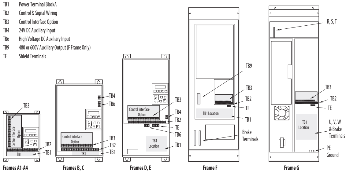
Figure 15 - 1336 PLUS Drive Power Terminal Block Locations
