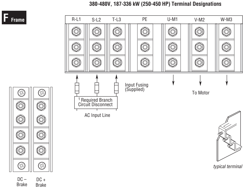
Figure 18 - 1336 PLUS Drive Power Terminal Blocks (F, G)
