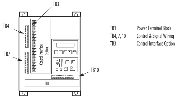
Figure 28 - 1336 IMPACT Drive Power Terminal Blocks (A1...A4)
