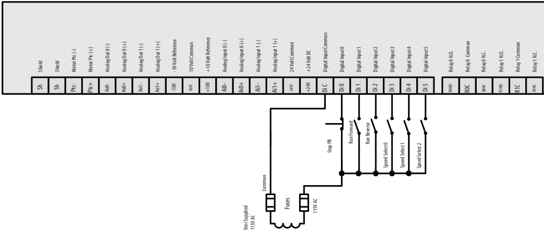
Figure 72 - 2-wire Control, Preset Speeds Wiring Example
