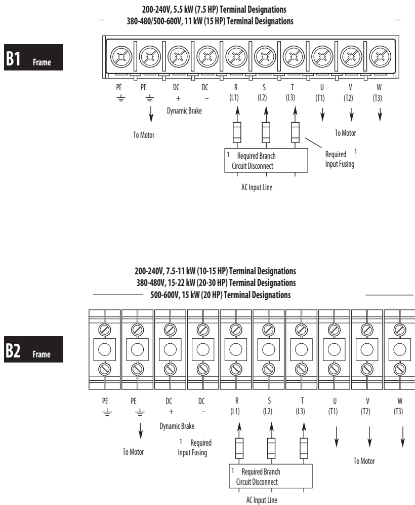
Figure 30 - 1336 IMPACT Drive Power Terminal Blocks (B1, B2)
