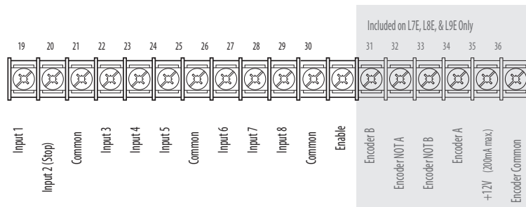
Figure 53 - 1336 IMPACT Drive “L” Option Terminals (TB3)
