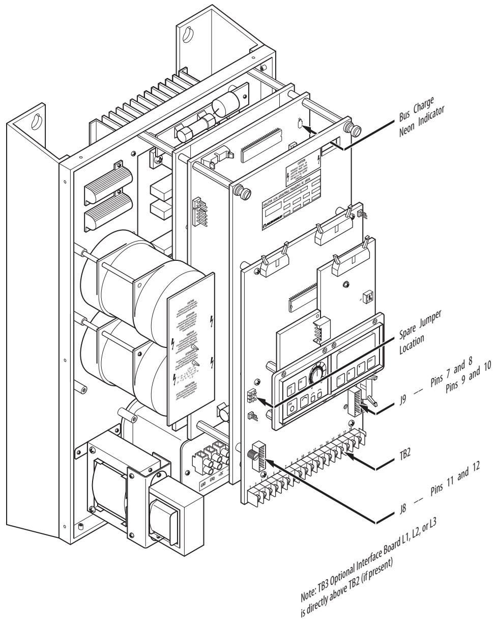
Figure 38 - 1336 CLASSIC Drive Terminal Blocks TB2 and TB3 Locations
